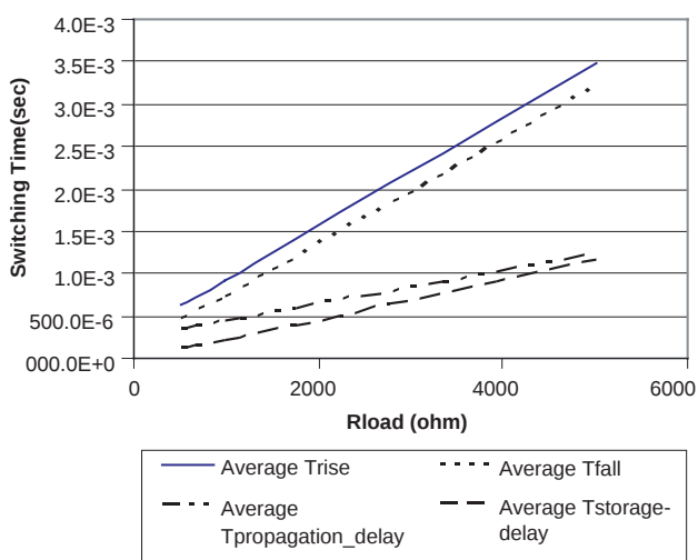
Switching Charecteristics (TA = 25C, Vcc = 3V)
