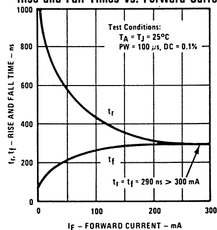
Rise and Fall Times vs. Forward Current
