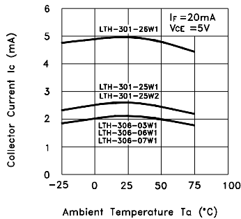
Fig.6 Collector Current vs. Ambient Temperature
