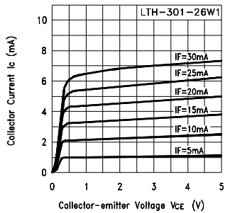
Fig.5 Collector Current vs. Collector-emitter Voltage
