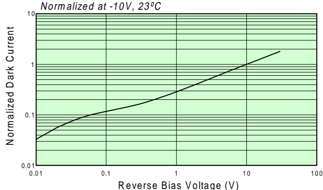
Typical Dark Current vs Reverse Bias
