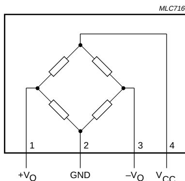
Fig.2 Simplified circuit diagram.
