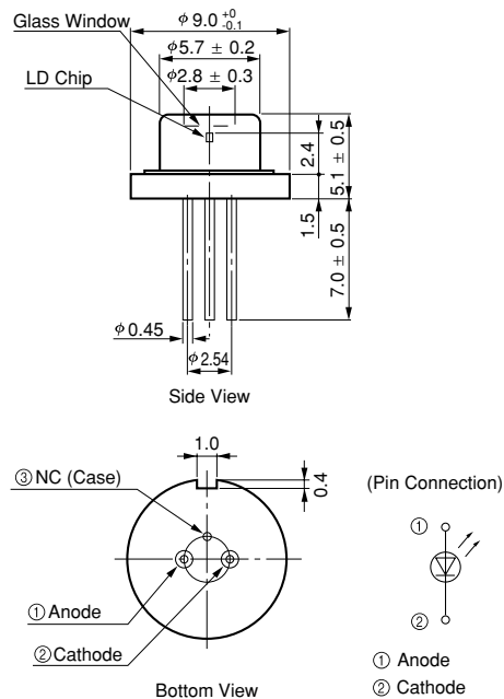
Figure 1: Dimensional Outline (Unit: mm)
