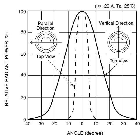
Figure 4: Typical Directivity
