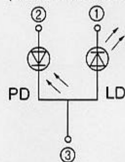
(Pin Connection)
