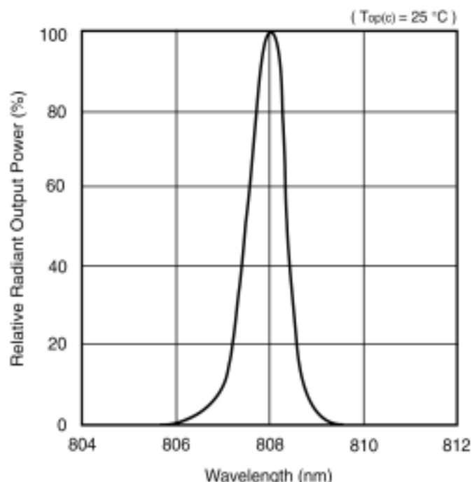
Figure 2: Emission Spectrum (Typ.)
