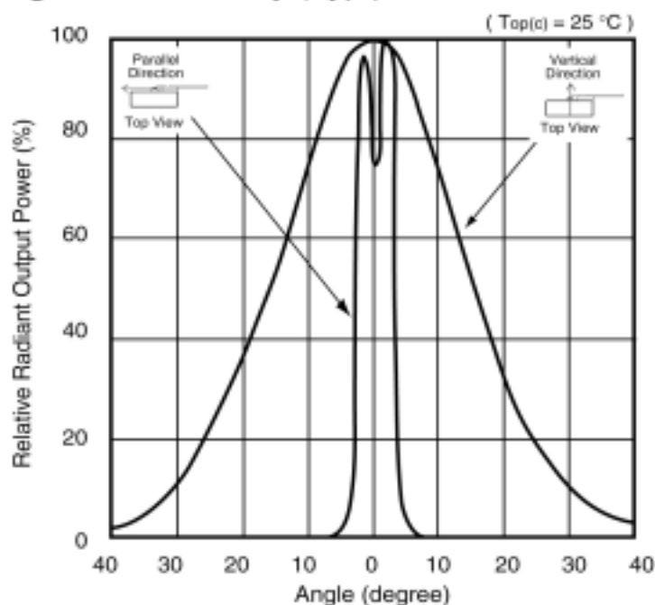
Figure 3: Directivity (Typ.)
