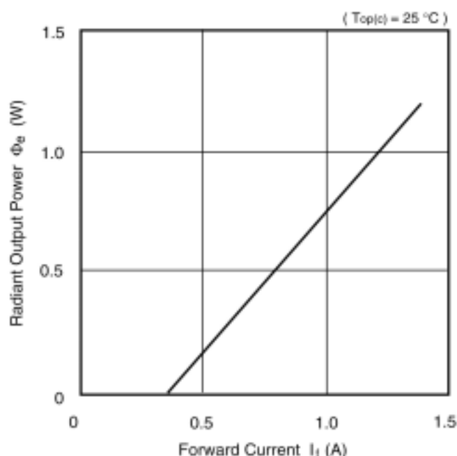
Figure 1: Radiant Output Power vs. Forward Current (Typ.)
