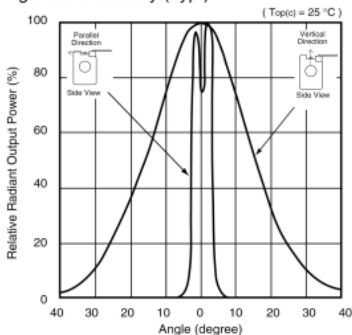
Figure 3: Directivity (Typ.)
