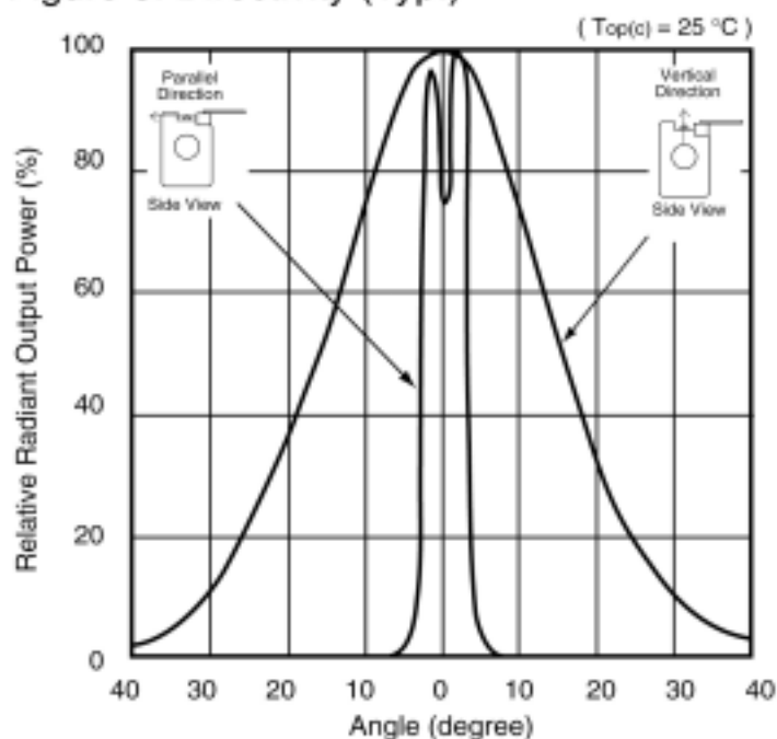
Figure 3: Directivity (Typ.)
