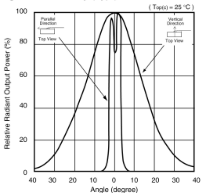
Figure 3: Directivity (Typ.)
