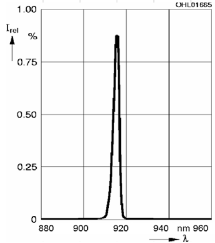
Optical spectrum, relative intensity I_{rel} vs. wavelength \lambda (15 W cw, 20 °C)
