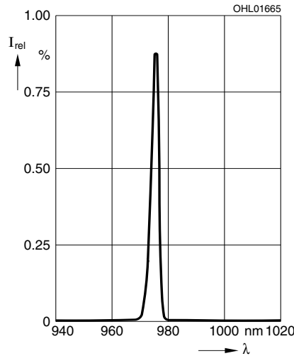
Optical spectrum, relative intensity I_{rel} vs. wavelength \lambda (15 W cw, 20 °C)
