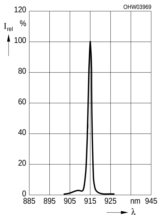
Optical Spectrum @ 180 W
