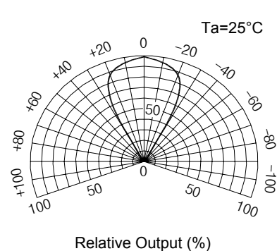
Sensitivity Diagram Angular Displacement
