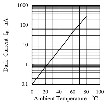
FIG.4 DARK CURRENT VS AMBIENT TEMPERATURE V_R=10 , E_e=0\text{ mW/cm}^2
