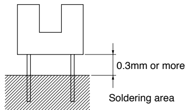
(GP1S196HCZ0F)
