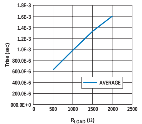
Figure 8. Rise time vs. R_{LOAD} .
