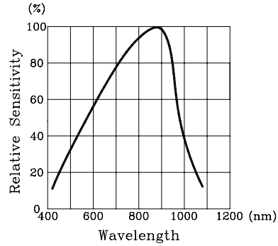
Spectral Sensitivity
