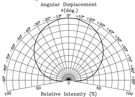
Radiation Diagram
