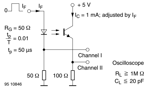
Fig. 10 - Pulse Diagram
