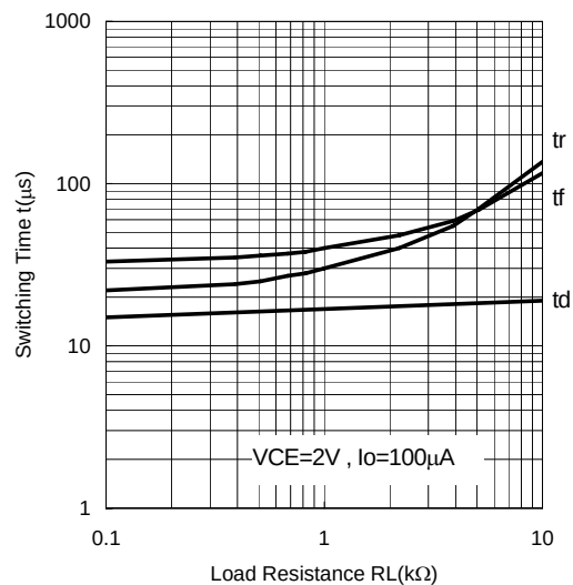
Switching Time vs. Load Resistance ( T_a=25^\circ\text{C} )
