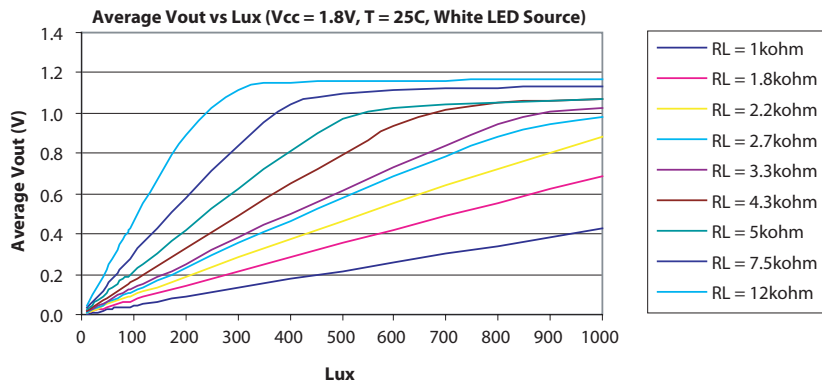
Figure 11. General Luminance vs Typical Output Voltage ( V_{CC} = 1.8V , T = 25^{\circ}C , Light Source = White LED)
