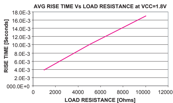
Figure 8. Average Rise Time Vs Load Resistance at Vcc = 1.8V
