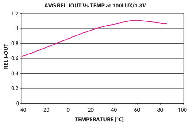
Figure 4. Average relative Iout Vs Temp (Vcc = 1.8V, T=25°C, 100 Lux)
