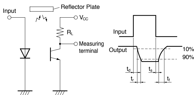
Fig.9 Test Circuit for Response Time
