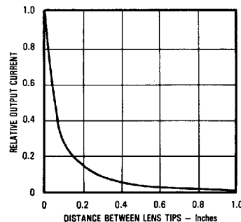
Coupling Characteristics OP145 and OP565
