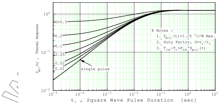
Figure 11. Thermal Response
