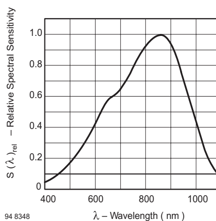
Figure 8. Relative Spectral Sensitivity vs. Wavelength
