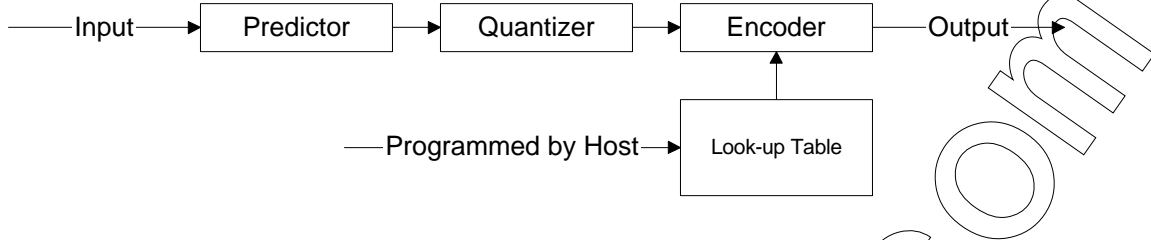
Figure 9. Structure of OmniCE
