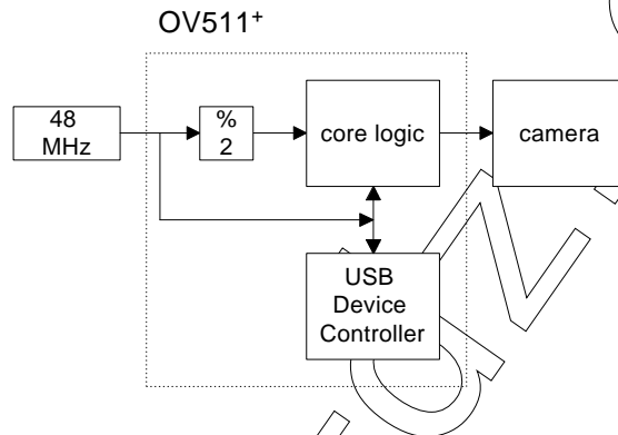
Figure 11. Clock Scheme of OV511 +
