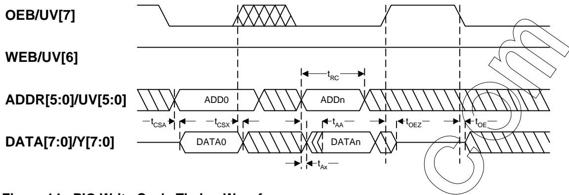
Figure 14. PIO Write Cycle Timing Waveforms
