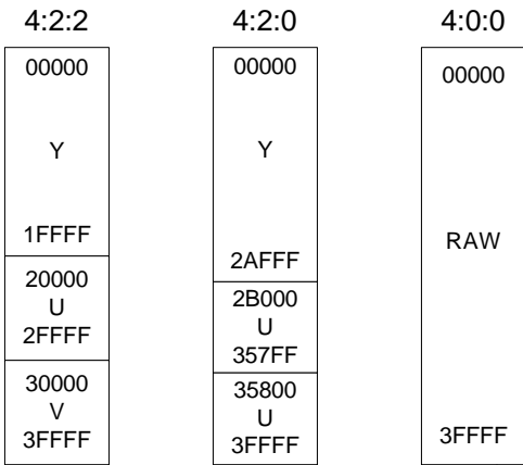
Figure 5. Memory Map
