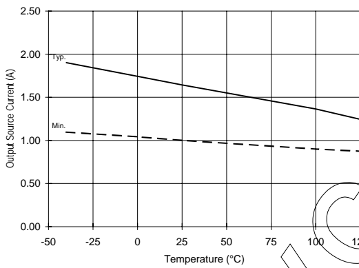
Figure 34A. Output Source Current vs. Temperature
