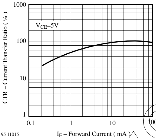
95 11015 Figure 13. Current Transfer Ratio vs. Forward Current
