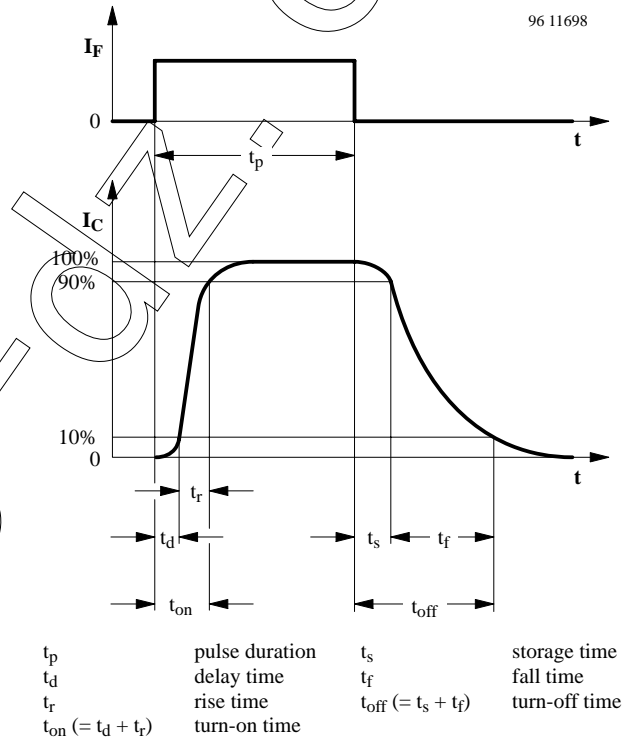
Figure 5. Switching times
