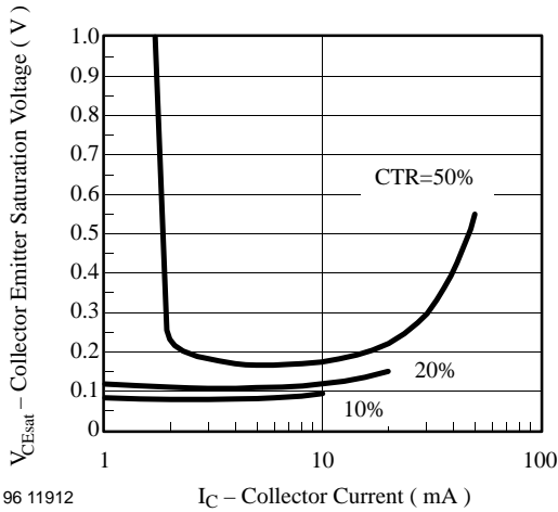
96 11912 Figure 12. Collector Emitter Saturation Voltage vs. Collector Current
