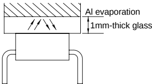
Test Condition and Arrangement for Collector Current
