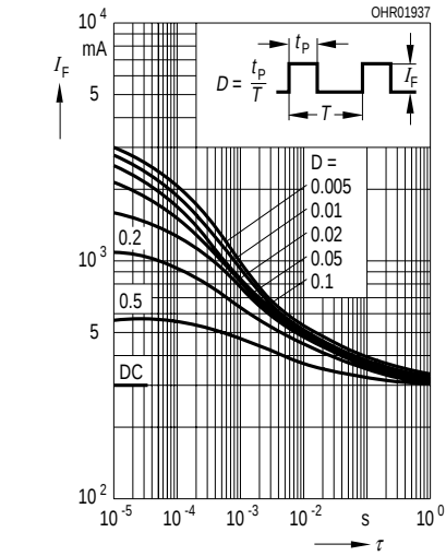
Permissible pulse handling capability I_F = f(\tau) , T_C = 25 \text{ °C} , R_{\text{thJC}} = 160 \text{ K/W} , duty cycle D = parameter
