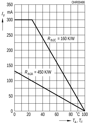
Max. permissible forward current SFH 400, SFH 402, I_F = f(T_A)
