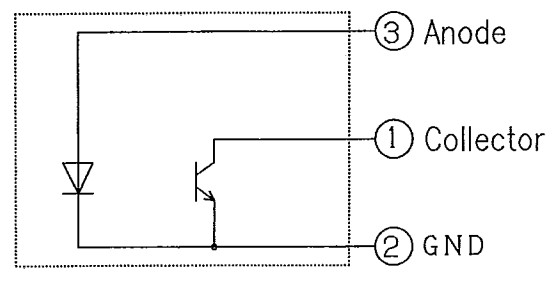
Internal Connection Diagram
