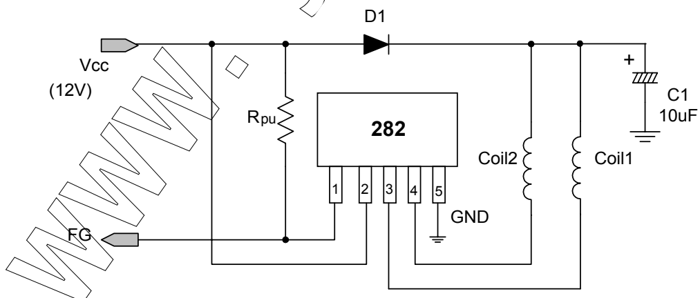
12V DC Brush-less Fan with FG output function
