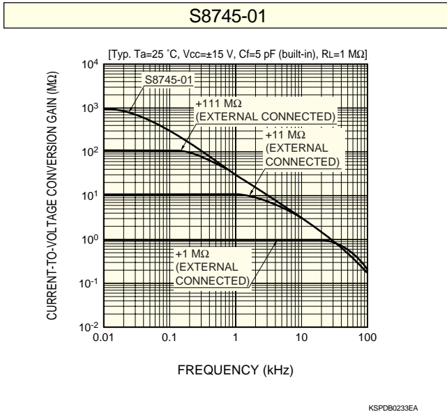
Figure 2 Gain-frequency characteristics
