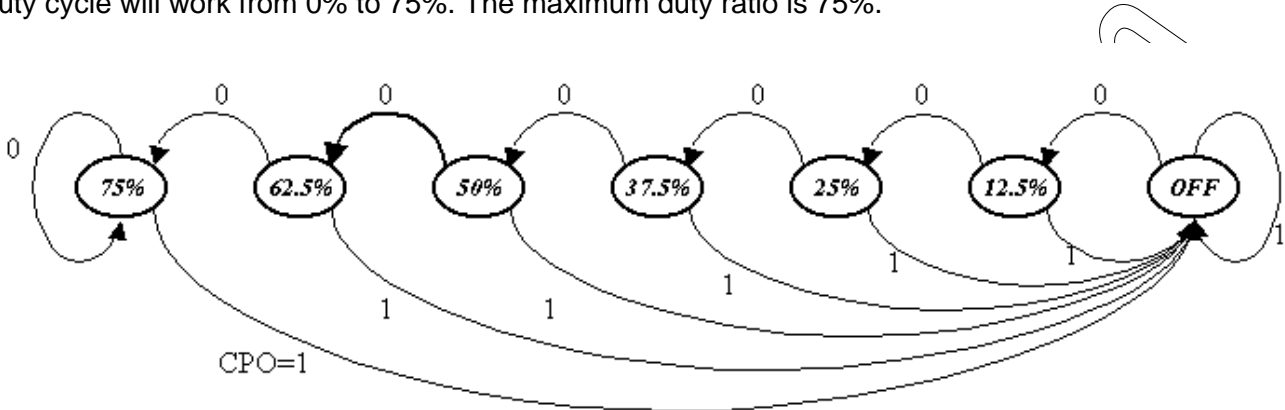
Fig 3 PWM Control state diagram
