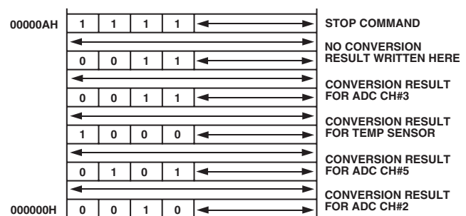
Figure 15. Typical External Memory Configuration Post ADC DMA Operation
