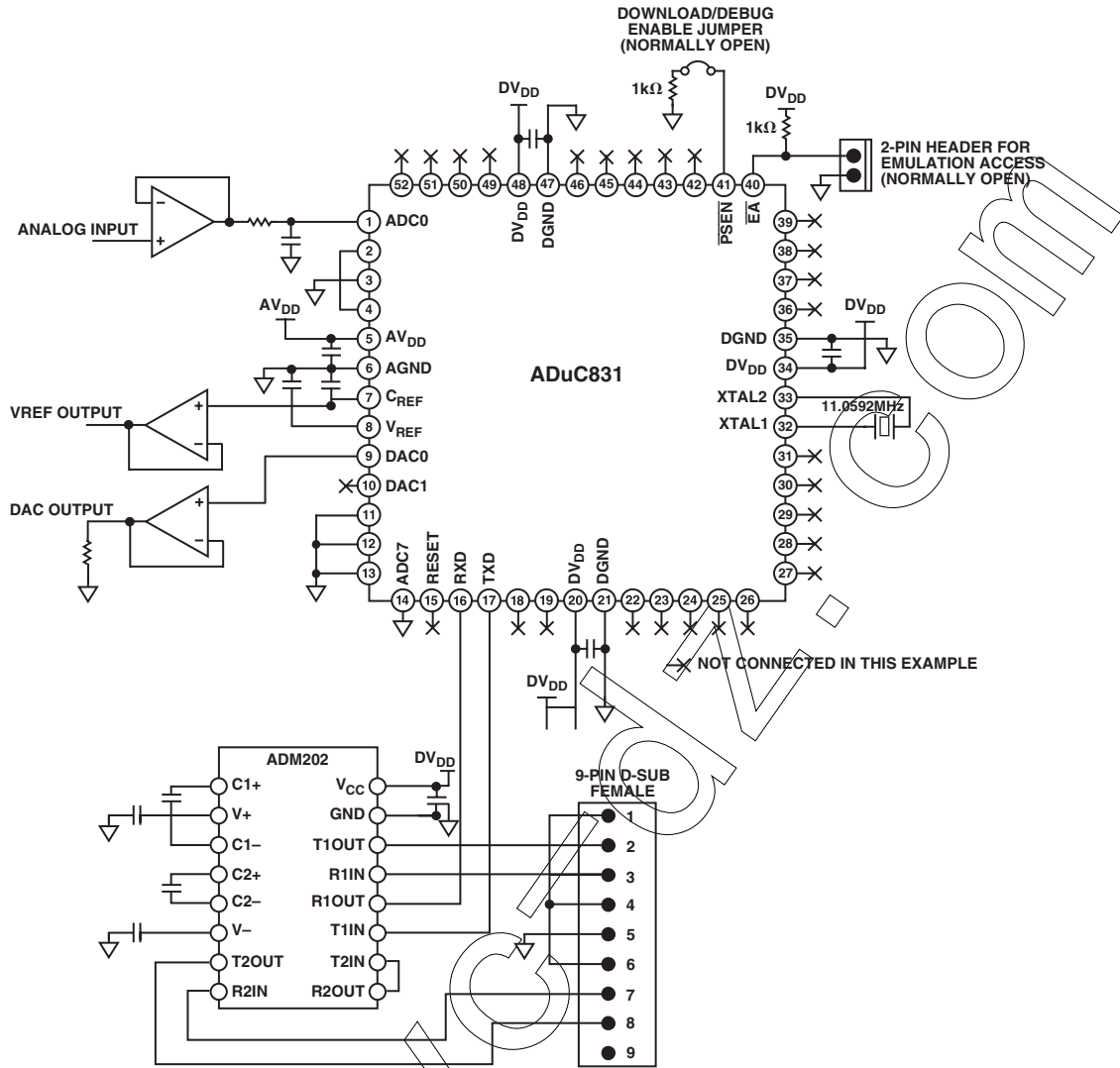
Figure 64. Example ADuC831 System (PQFP Package)
