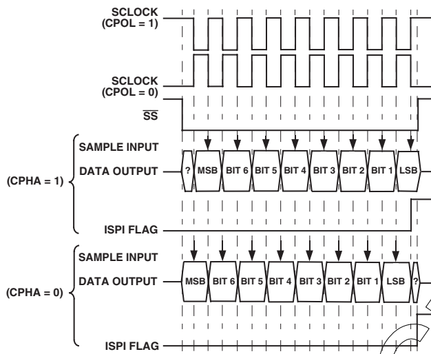
Figure 33. SPI Timing, All Modes
