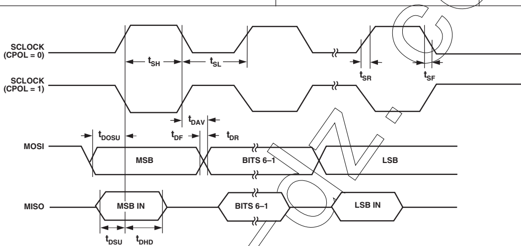
Figure 76. SPI Master Mode Timing (CPHA = 0)
