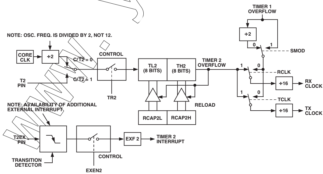
Figure 53. Timer 2, UART Baud Rates
