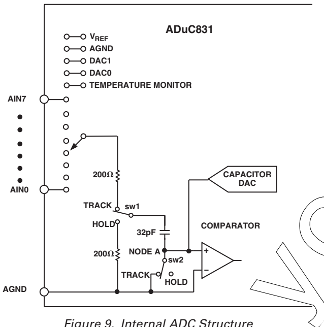
Figure 9. Internal ADC Structure
