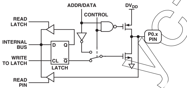
Figure 36. Port 0 Bit Latch and I/O Buffer
