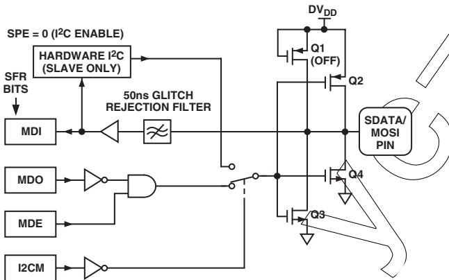
Figure 44. SDATA/MOSI Pin I/O Functional Equivalent in I 2 C Mode
