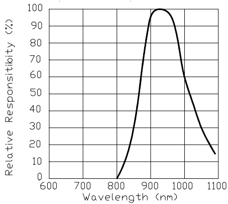
Fig.-4 Relative Spectral Sensitivity vs. Wavelength Direction
