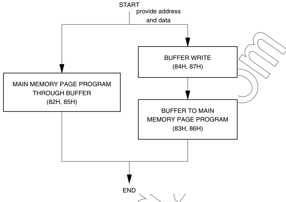
Figure 1. Algorithm for Sequentially Programming or Reprogramming the Entire Array
