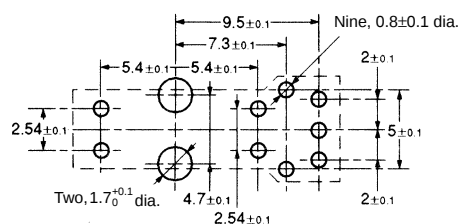
Recommended Mounting Holes
