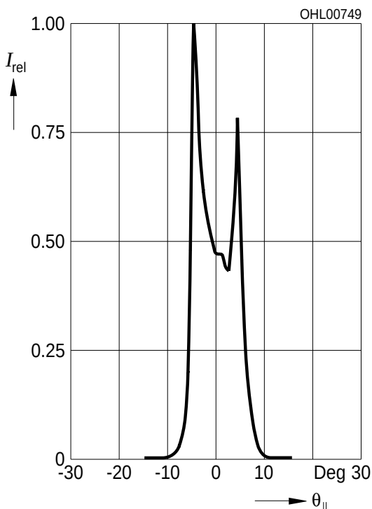
Far-field distribution parallel to junction I_{\text{rel}} vs. \theta_{\parallel} ( T_A = 25^\circ\text{C} , P_{\text{opt}} = 4\text{ W} )
