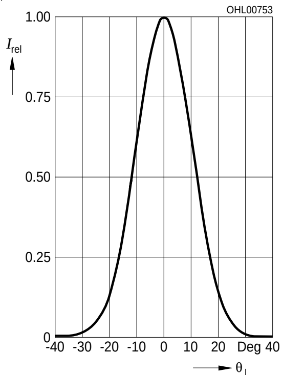
Far-field distribution perpendicular to junction I_{\text{rel}} vs. \theta_{\perp} ( T_A = 25^\circ\text{C} , P_{\text{opt}} = 4\text{ W} )
