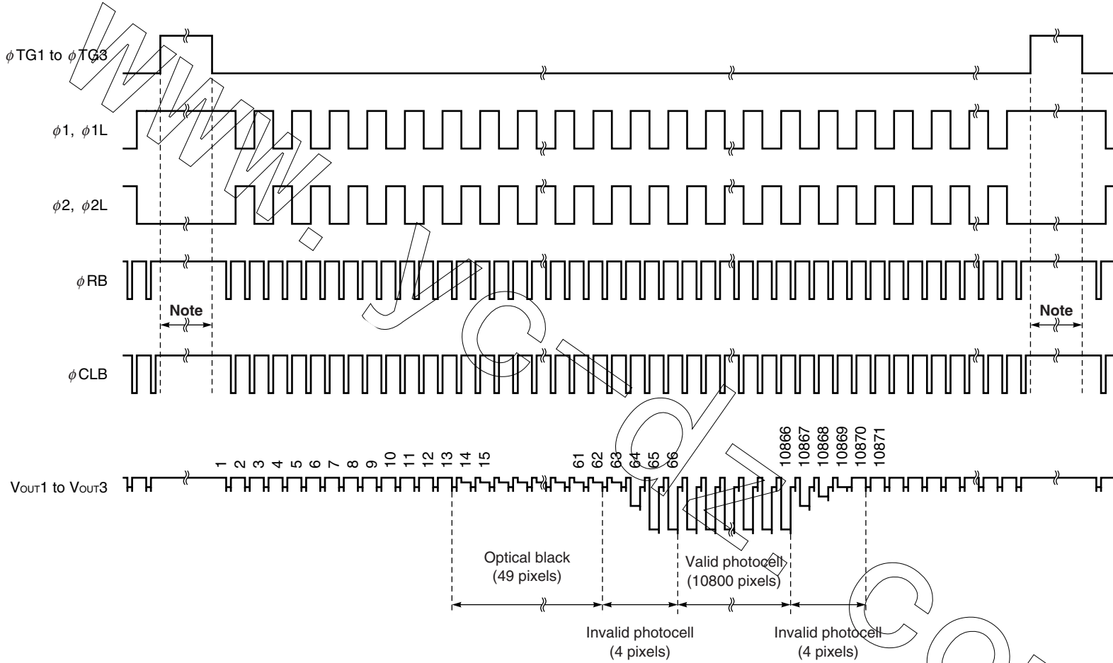
TIMING CHART 1-1 (Bit clamp mode, for each color)
