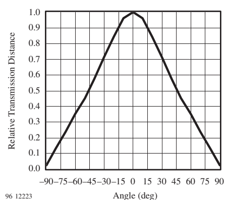
Figure 12. Directivity
