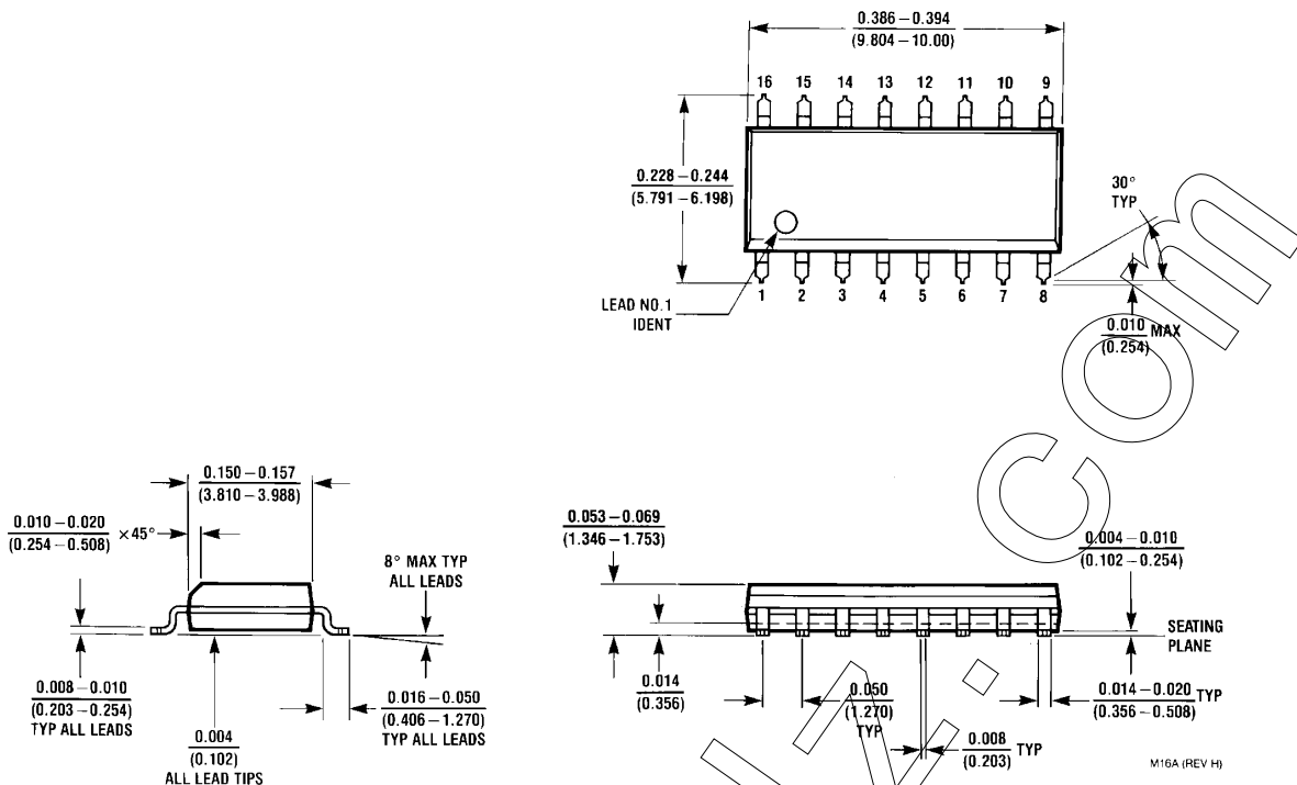
Small Outline Package Order Number DAC0808LCM NS Package Number M16A
